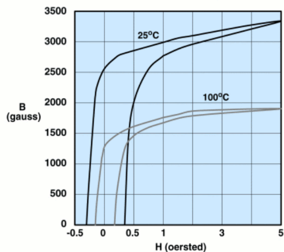
Hysteresis Loop
